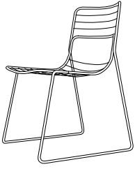
chair W510 L 560 H 780 seat 425
