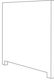
wide screen / tall W 500 L 1920 H 1500
