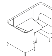
PULBW2H Pullman 2 Seat Booth Wide mm W 2250 D 1300 H 1300 Seat 450 inch W 88.5 D 51 H 51 Seat 18
