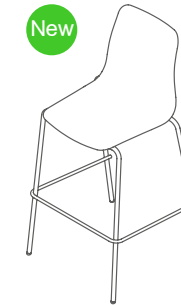
New POLLYBSB4L polly barstool 4 leg metric (mm) W568 D536 H1105 Seat 750 imperial (in) W22.5 D21 H43.5 Seat 29.5
