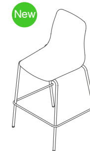
New POLLYCHBSB4L polly counter height stool 4 leg metric (mm) W568 D536 H1005 Seat 650 imperial (in) W22.5 D21 H39.5 Seat 25.5
