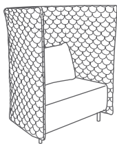
CLOQ15H cloud quilt 1.5 seat sofa with high back and black straight legs metric (mm) W1100 D750 H1300 Seat 400 imperial (in) W43.5 D29.5 H51 Seat 15.5
